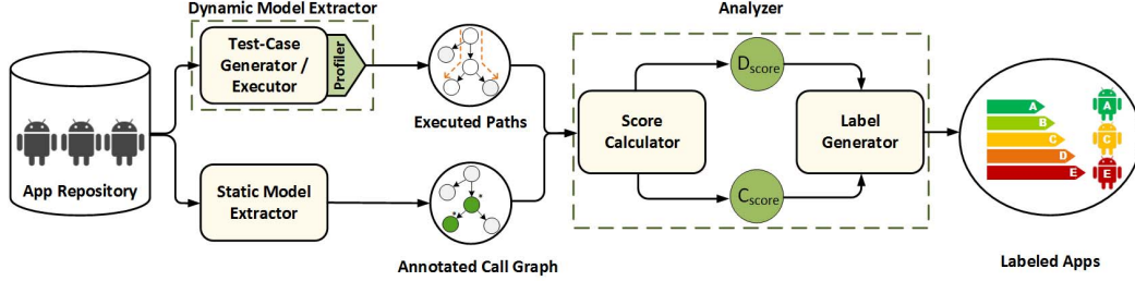
Fig. 2: EcoDroid Framework.
