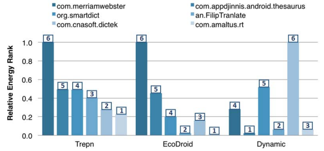
Fig. 5: Visualization of rankings provided by Trepan, EcoDroid, and dynamic approach.
